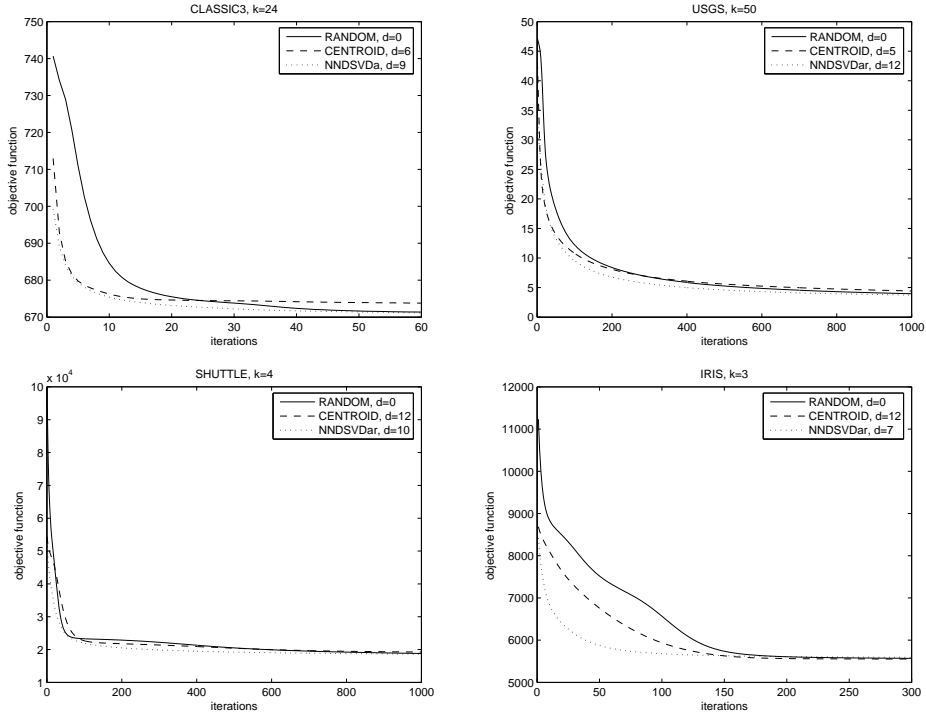
Fig. 2. Algorithm MM for datasets CLASSIC3, USGS, SHUTTLE, IRIS.
