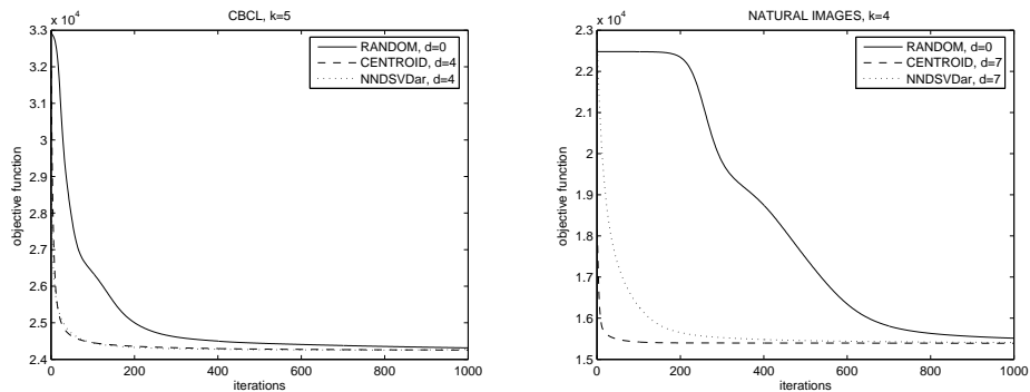
Fig. 7. Algorithm GD-CLS with \lambda = 0.01 for datasets CBCL and NATURAL IMAGES.
