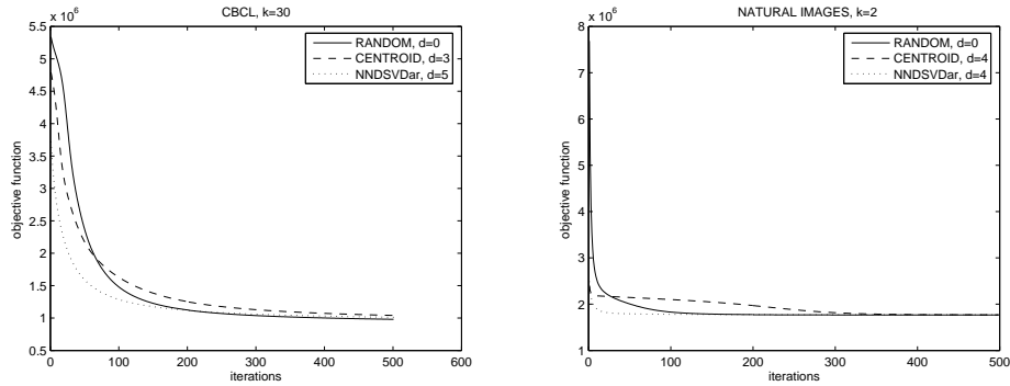
Fig. 5. Algorithm AD for datasets CBCL and NATURAL IMAGES.
