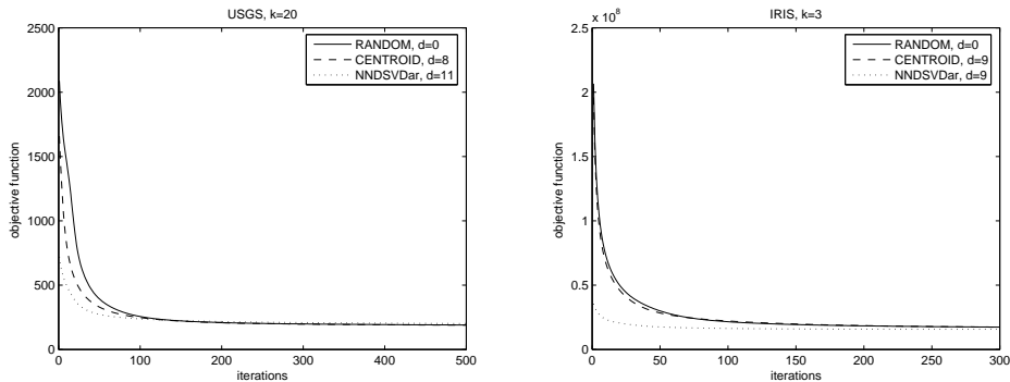
Fig. 6. Algorithm CNMF with \alpha = \beta = 0.5 for datasets USGS, IRIS.
