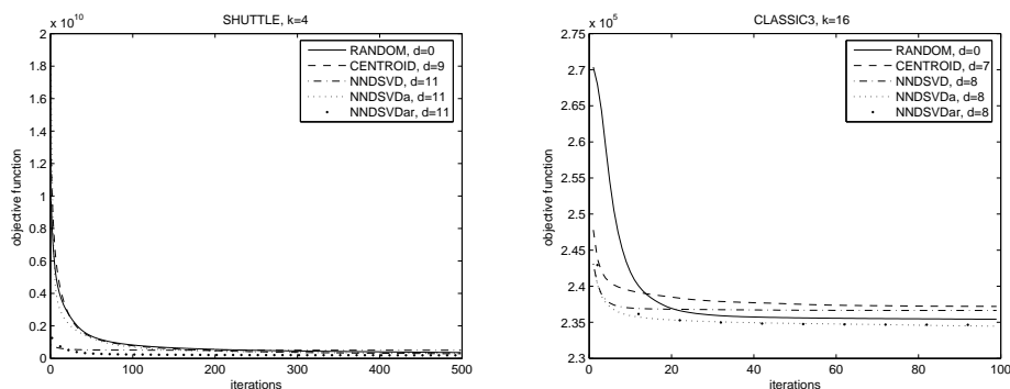
Fig. 9. NNDSVD, NNDSVdA, NNDSVDar and CENTROID on CNMF ( \alpha = \beta = 0.5 ) for datasets SHUTTLE and CLASSIC3.
