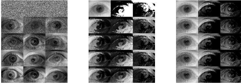
Fig. 4. Progress of approximation on iris dataset using MM: Random (left); NNDSVDar (center); NNDSVD (right). Rows correspond to 0, 20, 40, 60 and 80 iterations using k = 3 .
