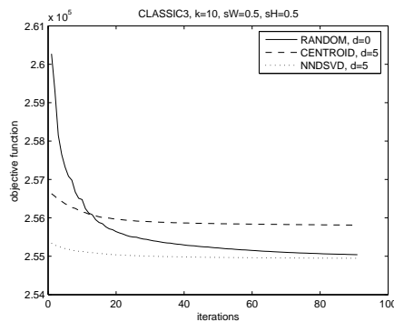
Fig. 8. Sparse NMF algorithm, nmf_sc , for dataset CLASSIC3.
